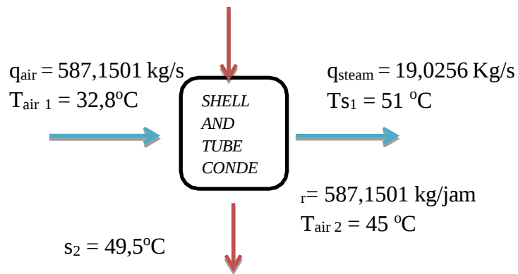
Gambar 2. Aliran Proses Shell and Tube Kondensor
