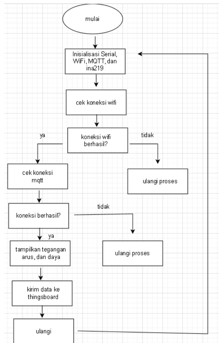
Gambar 3. Flowchart program
